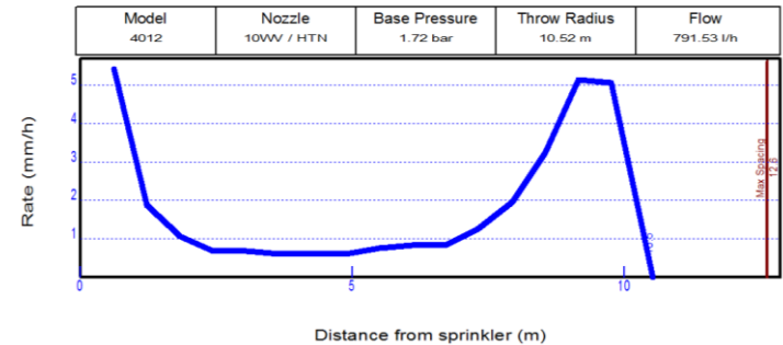
Sprinkler Profile
