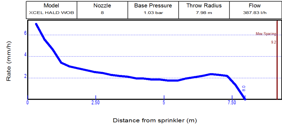
Sprinkler Profile
